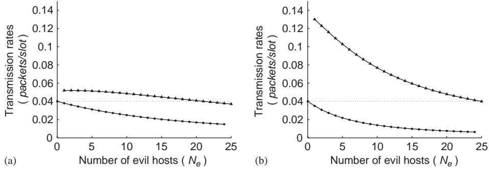
Fig. 2. The transmission rates for the stateless model as a function of the number of evil hosts, N_e , in a network with N = 25 players. (a) has been evaluated using an evil probability p = 0.1 . (b) p = 0.25 . The line with solid triangles represents the evil rate R_e(N, N_e, p) . The line with solid circles represents the fair rate R_f(N, N_e, p) . The dotted line indicates the yield of the all-fair situation, R_f(N, 0, p) . As can be observed, in both cases the game is a Tragedy of the Commons because there is always an incentive for a new player to become evil and the final rate of evil hosts in the Nash equilibrium, R_e(N, N, p) , is always under the initial yield of fair players R_f(N, 0, p) .
