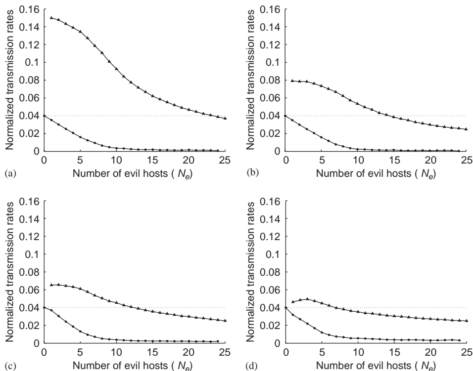
Fig. 9. The curves show the normalized transmission rates obtained from the simulations as a function of the number of evil hosts, N_e , in a network with N = 25 players. Curve (a) has been evaluated using a buffer size m = 2 . In (b), m = 10 . In (c) m = 30 and in (d), m = 100 . The line with solid triangles represents the normalized evil rate. In solid circles we have the normalized fair rate. The dotted line indicates the initial yield of fair hosts. As can be observed, in all cases, the behavior of the simulations is similar to the predictions of the theoretical model.
