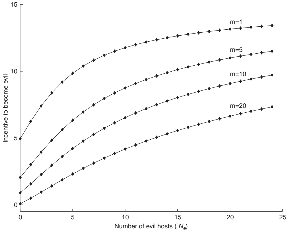
Fig. 8. The incentive to become evil as a function of the number of evil hosts in a network with N = 25 hosts. As can be observed, the incentive decreases when m grows. In the simulations the evil probability has been fixed to a value p = 0, 6 .
