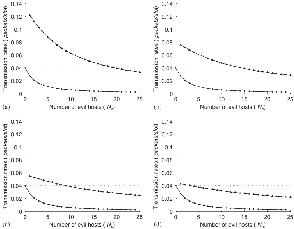
Fig. 7. Transmission rates for the Markovian model as a function of the number of evil hosts, N_e , in a network with N = 25 players. The evil probability is fixed to p = 0.6 in all graphs. Curve (a) has been evaluated using a buffer size m = 5 . In (b), m = 10 . In (c) m = 15 and in (d), m = 20 . The evil rate R_T(N, N_E, p, m) is represented by solid triangles. In circles we have the fair rate R_F(N, N_e, p, m) . The dotted line indicates the initial yield of the all-fair situation, R_F(N, 0, p, m) . As can be observed, in all cases the game is a Tragedy of the Commons, but its effect is more remarkable when the buffer size, m , increases.
