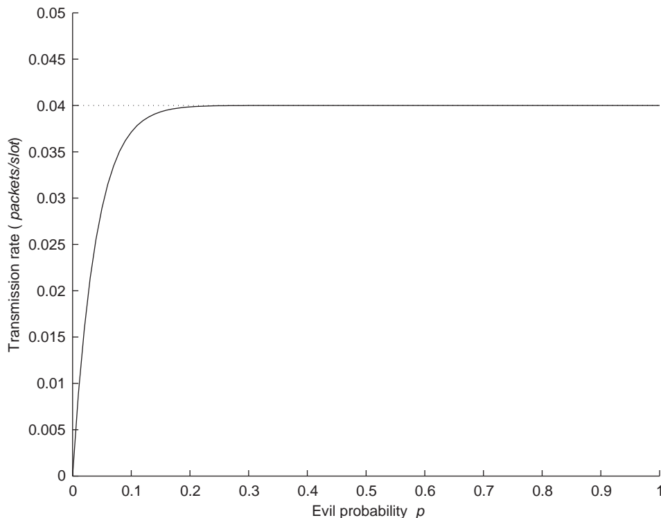
Fig. 3. Increase in the final evil rate in the Nash equilibrium, R_e(N, N, p) , with p . The dashed line represents the initial fair rate R_f(N, 0, p) . The simulation has been performed in a network of N = 25 hosts.
