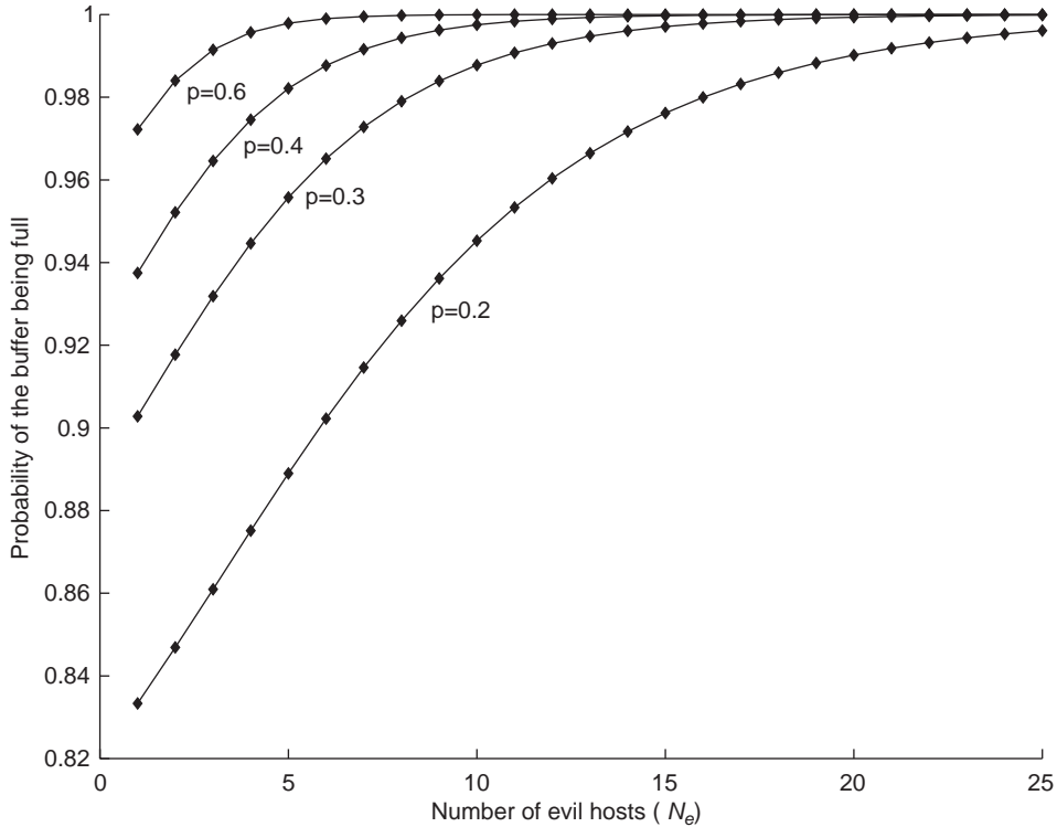
Fig. 5. The stationary probability X_m of the buffer being full as a function of the number of evil hosts N_e for 4 different values of the evil selfishness p . The size of the network has been fixed to N = 25 . As can be observed, even for moderate values of p , X_m rapidly goes to 1.
