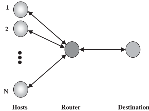
Fig. 1. The interconnecting topology of the network we use in the proposed model. N hosts try to access a common communication link through a router. This router has a finite buffer which drops packets when it is full. All lines have a capacity of one packet per time slot (or step).
