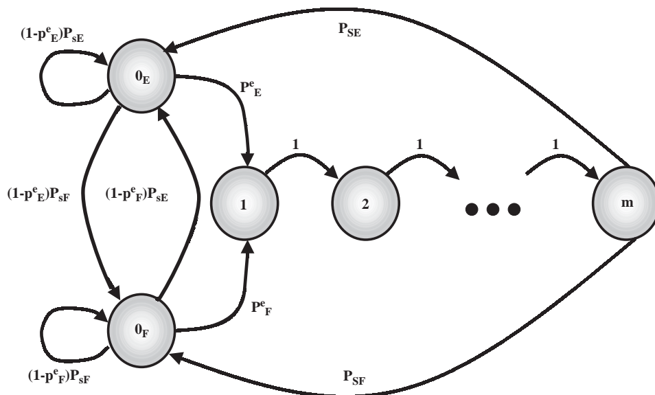
Fig. 6. A schema of the Markov Chain proposed to track the evolution of packets from a given evil host in the router buffer. In states 0_E and 0_F there are no useful packets in the buffer and the host is trying to inject one. The difference between these two states is in the type of current slot: E in the former case and F in the latter. In the rest of the cases, the state reflects the position of the useful packet within the buffer. Observe that p_{sF} = \frac{N_f}{N} is the probability of the next slot to be fair while p_{sE} = \frac{N_e}{N} is the probability of the next slot to be evil. Once the packet is in the FIFO buffer, its probability to pass to the next state is always 1. When the packet is delivered (state m ), the host is immediately notified and it starts sending a new packet in states 0_E or 0_F depending on whether the subsequent slot is evil or fair.
