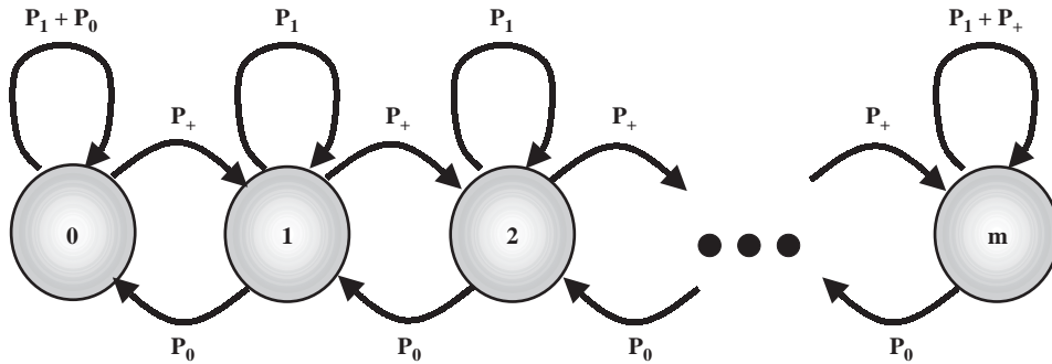
Fig. 4. The Markov Chain proposed to model the occupation of the router buffer. State i corresponds to a situation where there are exactly i packets in the buffer, p_0 is the probability of 0 packets being issued by hosts in a given time slot, p_1 is the probability of 1 packet being issued and p_+ is the probability of more than one packet trying to get into the buffer in that time slot. As an approximation, we consider that the buffer occupation can only increase in steps of one packet. The probability of the buffer being full corresponds to the probability of state m .
